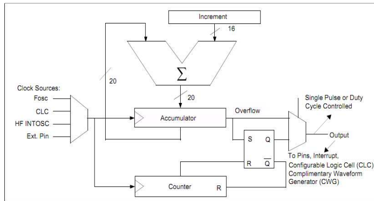
Figure 2: Internal Block Diagram of NCO Module
