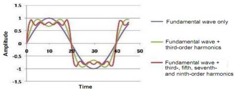
Figure 5: Frequency Wave Components in Square
