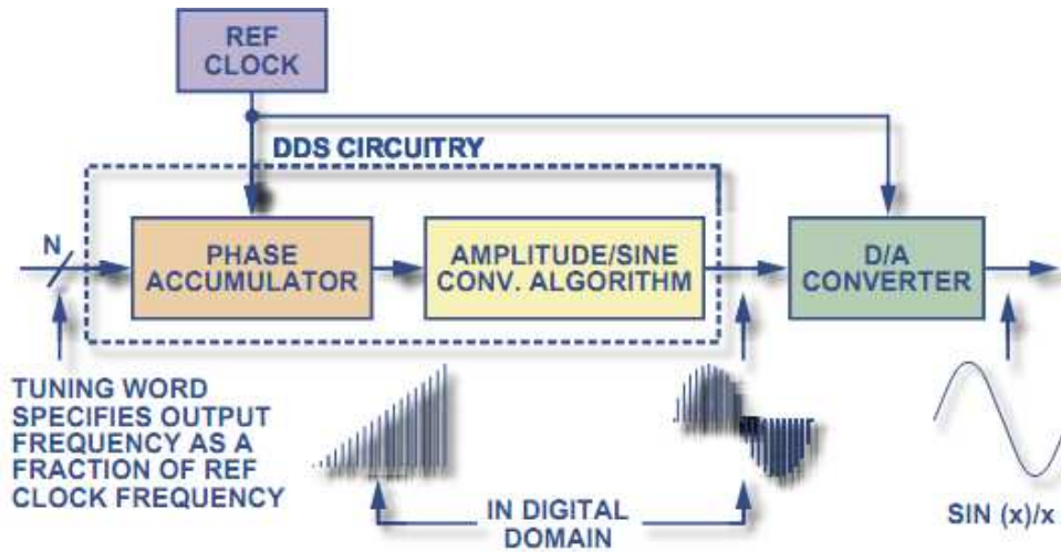
Figure 4: Signal Flow through the DDS Architecture
