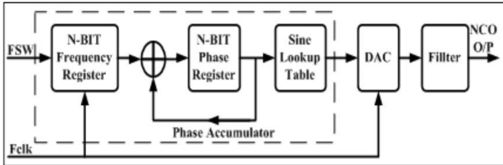
Figure 1: Block Diagram of NCO System
