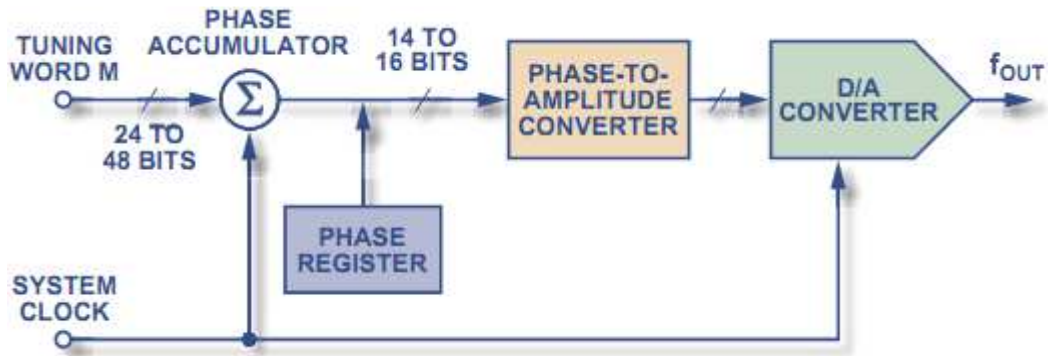
Figure 3: Internal Circuit of Direct Digital Synthesizer
